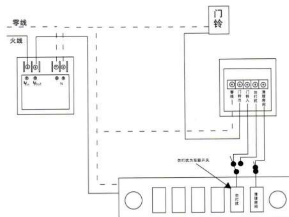
3916 (银) 勿打扰 请打扫 三合一门铃开关 Door bell switch with donot disturband make up room
