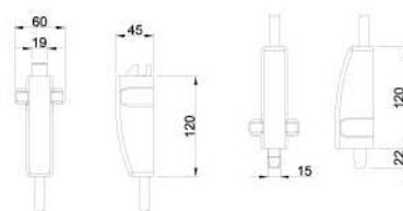
Top and bottom bolt for CMP436
