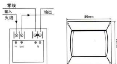
0309T / 0309M(香槟) 识别感应卡取电开关 RF card Energy-saving Switch
